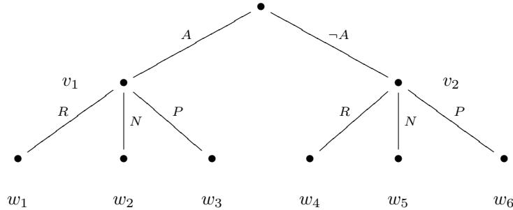
Figure 2: Game Model for Punishing and Rewarding Hearer Actions
