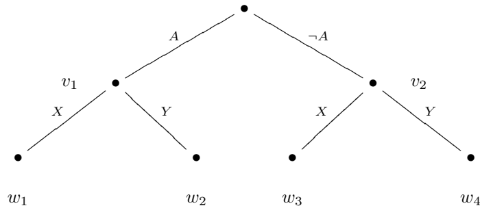
Figure 1: Sequential Game with Potential for Commitment
